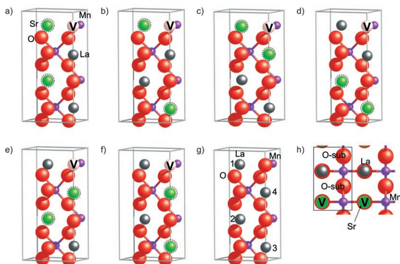
Figure 1. a)–f) \text{La}_{0.5}\text{Sr}_{0.5}\text{MnO}_3(110) surface models (A, B, C, D, E, and F, respectively) and g) undoped \text{LaMnO}_3(110) . Dashed circles and V denote Sr cations and doubly charged oxygen vacancies, respectively. h) Top view of adsorption sites on LaMn-terminated \text{La}_{0.5}\text{Sr}_{0.5}\text{MnO}_3(110) (surface model F). The rectangle represents a supercell for surface calculations; it contains a total of 19 ions (two La, two Sr, four Mn, and 11 O ions) and an oxygen vacancy. La gray, Sr green, Mn purple, O red.
